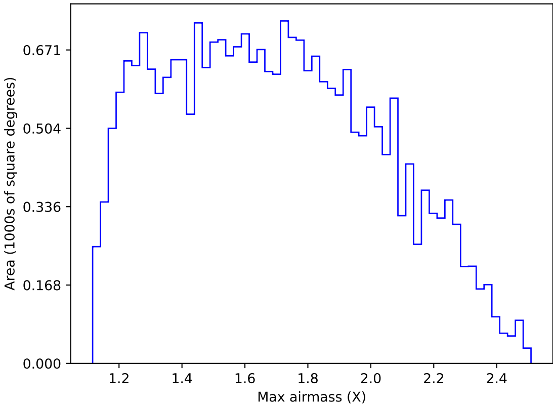
too_elab_heavy_r64_d2_gz_v3.4_10yrs Yr 1 g band: Max airmass
