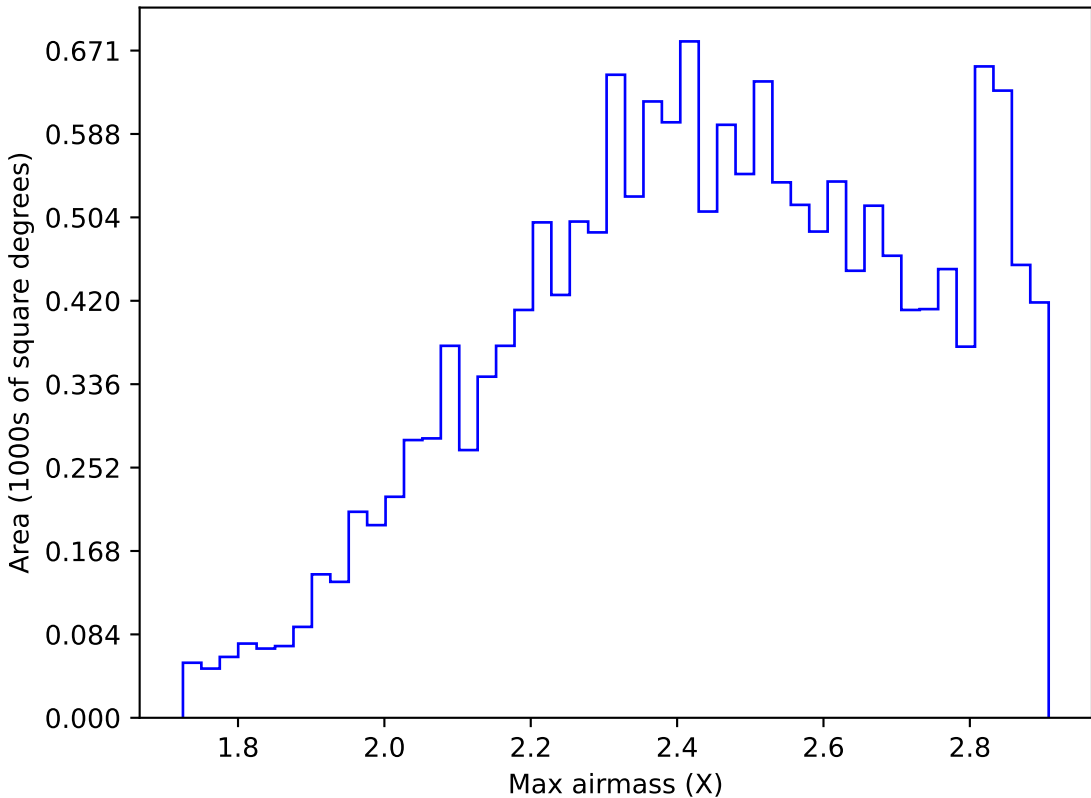
too_elab_heavy_r64_d2_gz_v3.4_10yrs WFD z band: Max airmass
