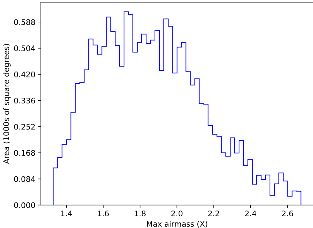
too_elab_heavy_r64_d2_gz_v3.4_10yrs WFD u band: Max airmass
