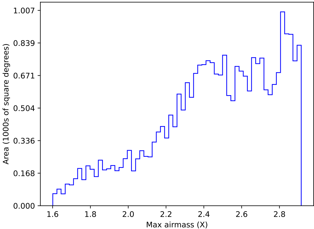
too_elab_heavy_r64_d2_gz_v3.4_10yrs All sky i band: Max airmass
