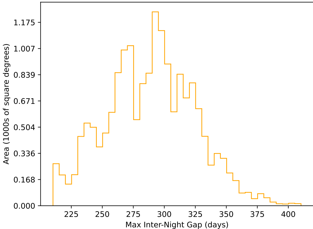
too_elab_heavy_r64_d2_gz_v3.4_10yrs WFD r band: Max Inter-Night Gap
