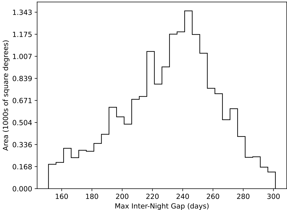
too_elab_heavy_r64_d2_gz_v3.4_10yrs WFD all bands: Max Inter-Night Gap
