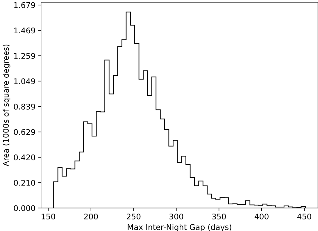
too_elab_heavy_r64_d2_gz_v3.4_10yrs All sky all bands: Max Inter-Night Gap
