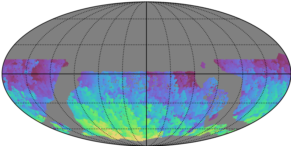
too_elab_heavy_r64_d2_gz_v3.4_10yrs WFD u band: Max HA
