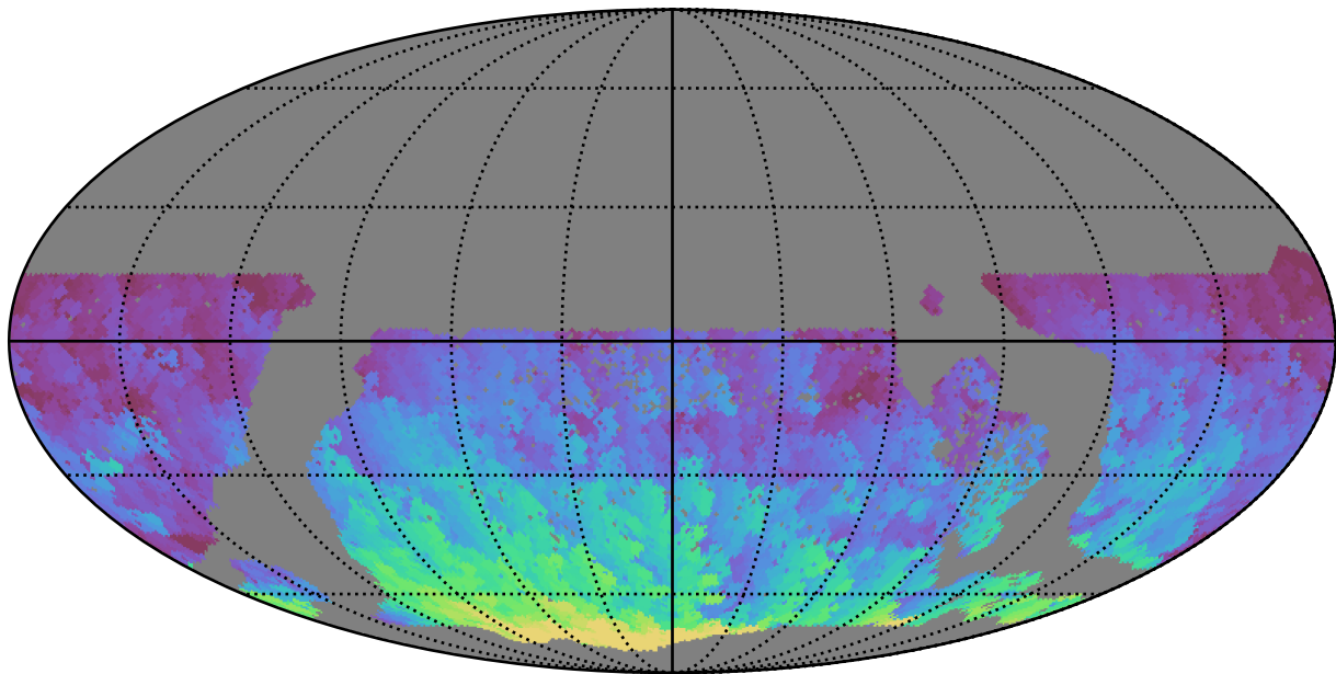
too_elab_heavy_r64_d2_gz_v3.4_10yrs WFD r band: Max HA
