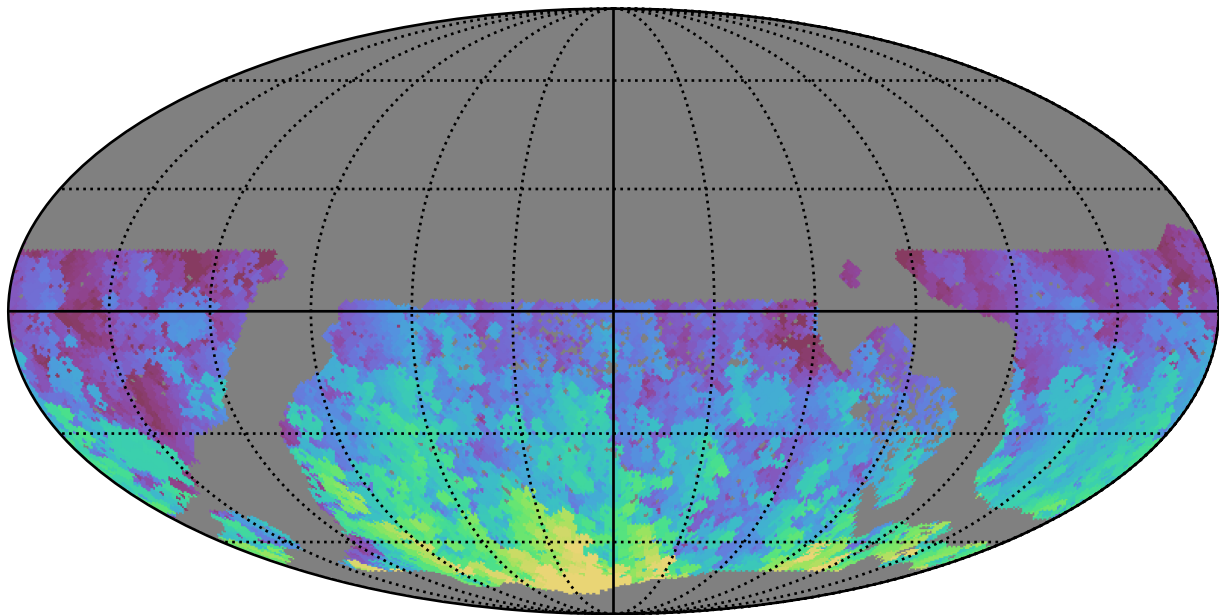
too_elab_heavy_r64_d2_gz_v3.4_10yrs WFD g band: Max HA
