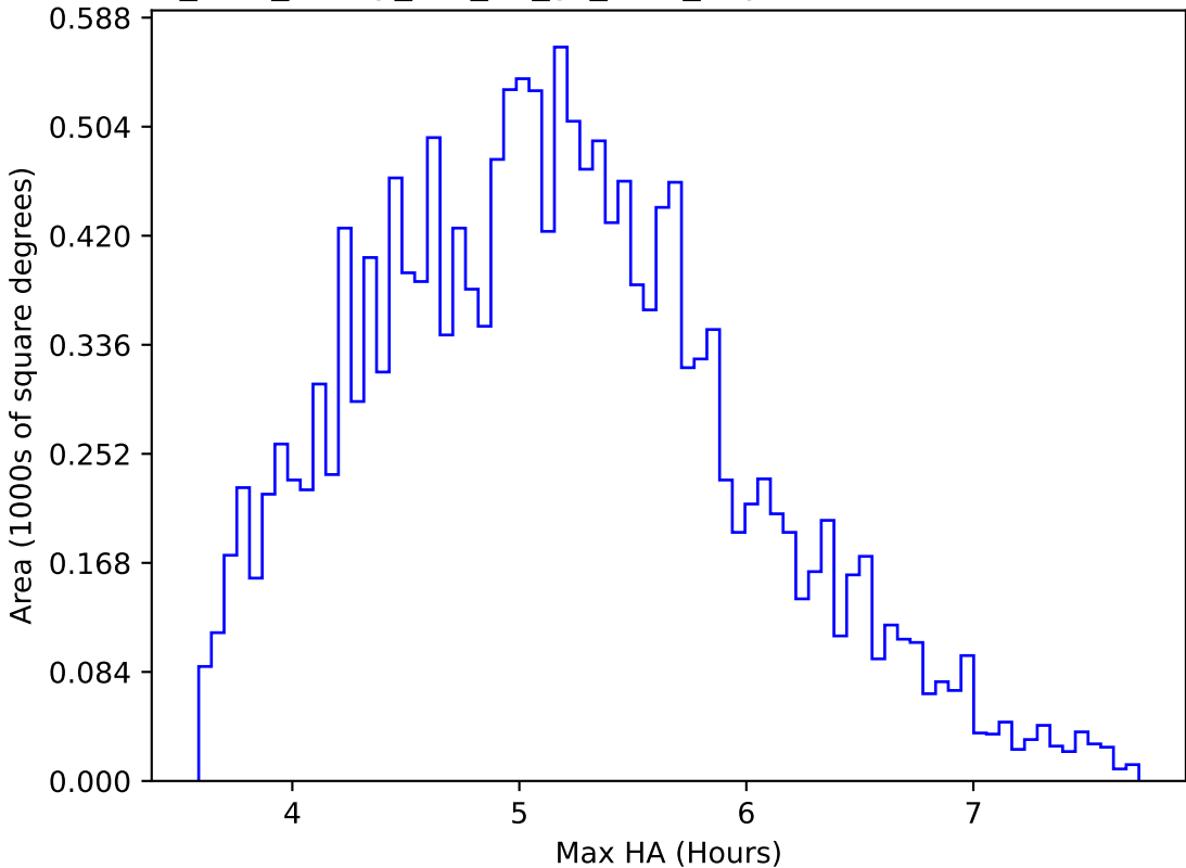
too_elab_heavy_r64_d2_gz_v3.4_10yrs WFD all bands: Max HA
