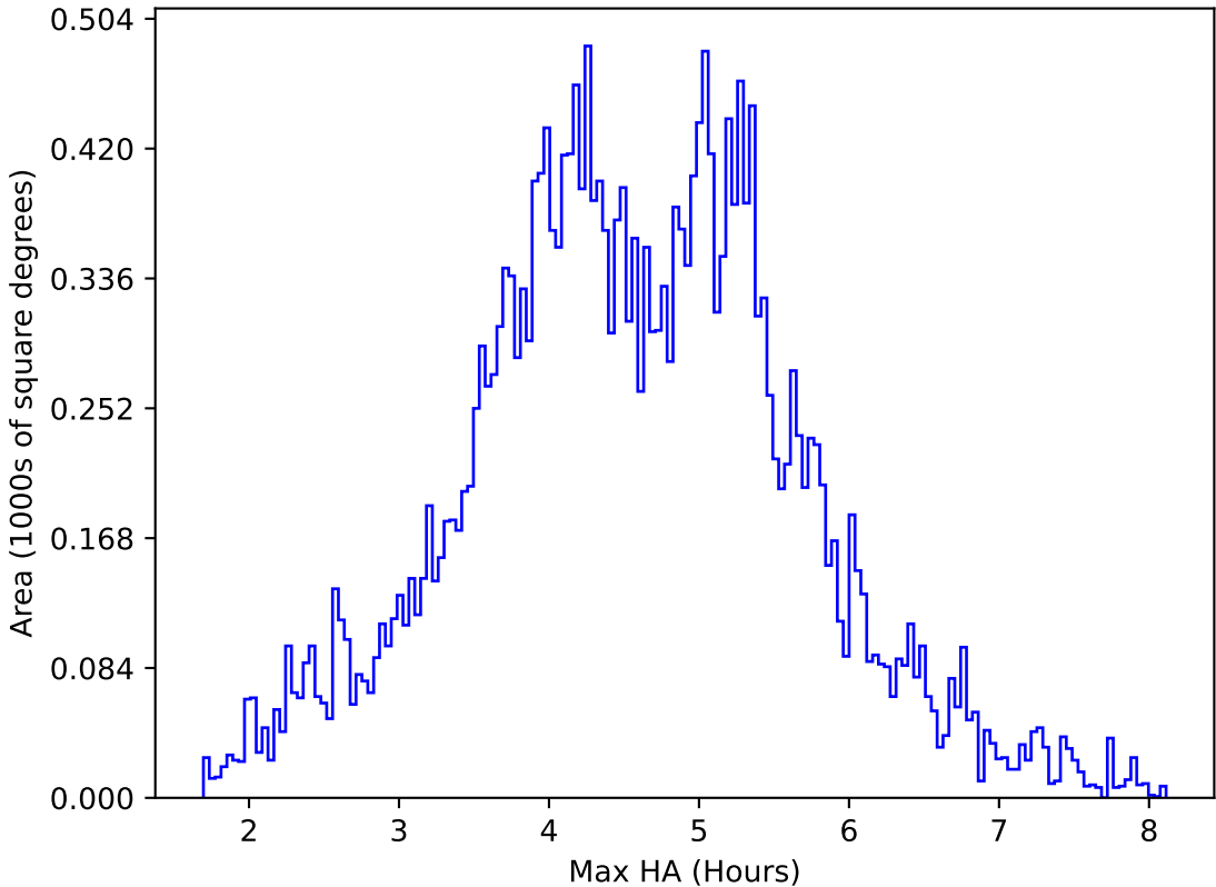
too_elab_heavy_r64_d2_gz_v3.4_10yrs All sky z band: Max HA
