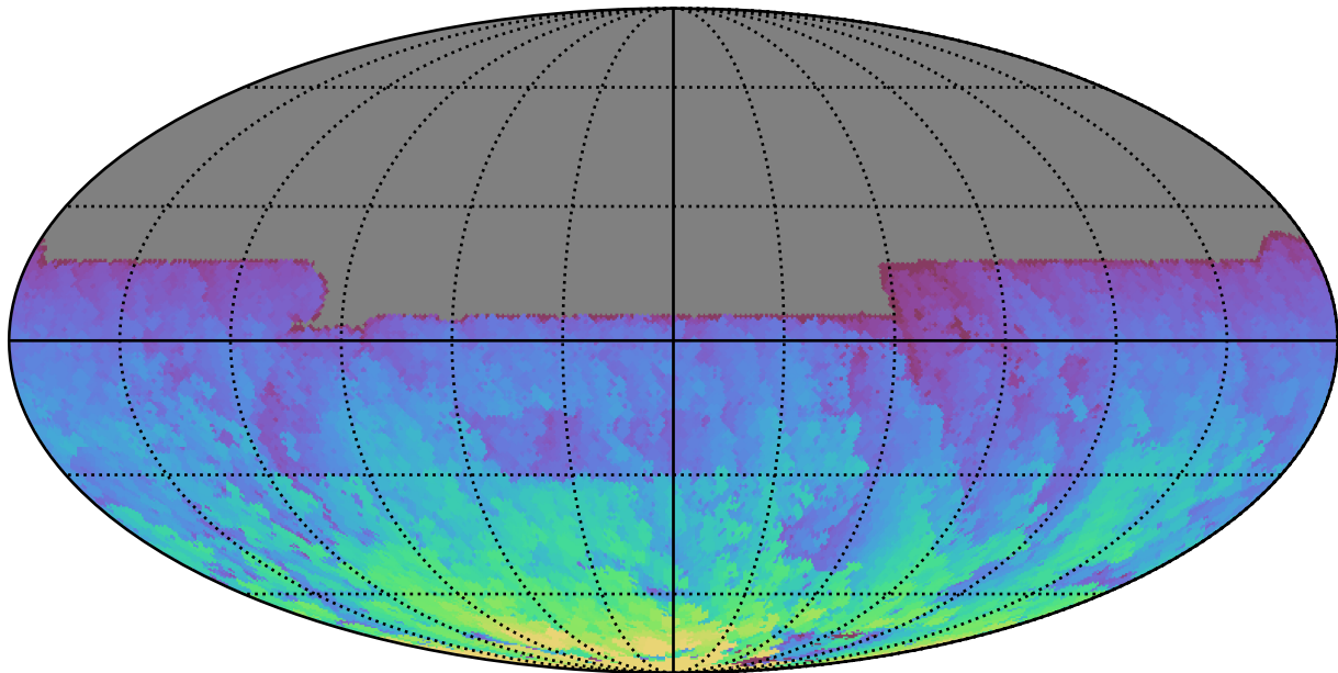
too_elab_heavy_r64_d2_gz_v3.4_10yrs All sky y band: Max HA
