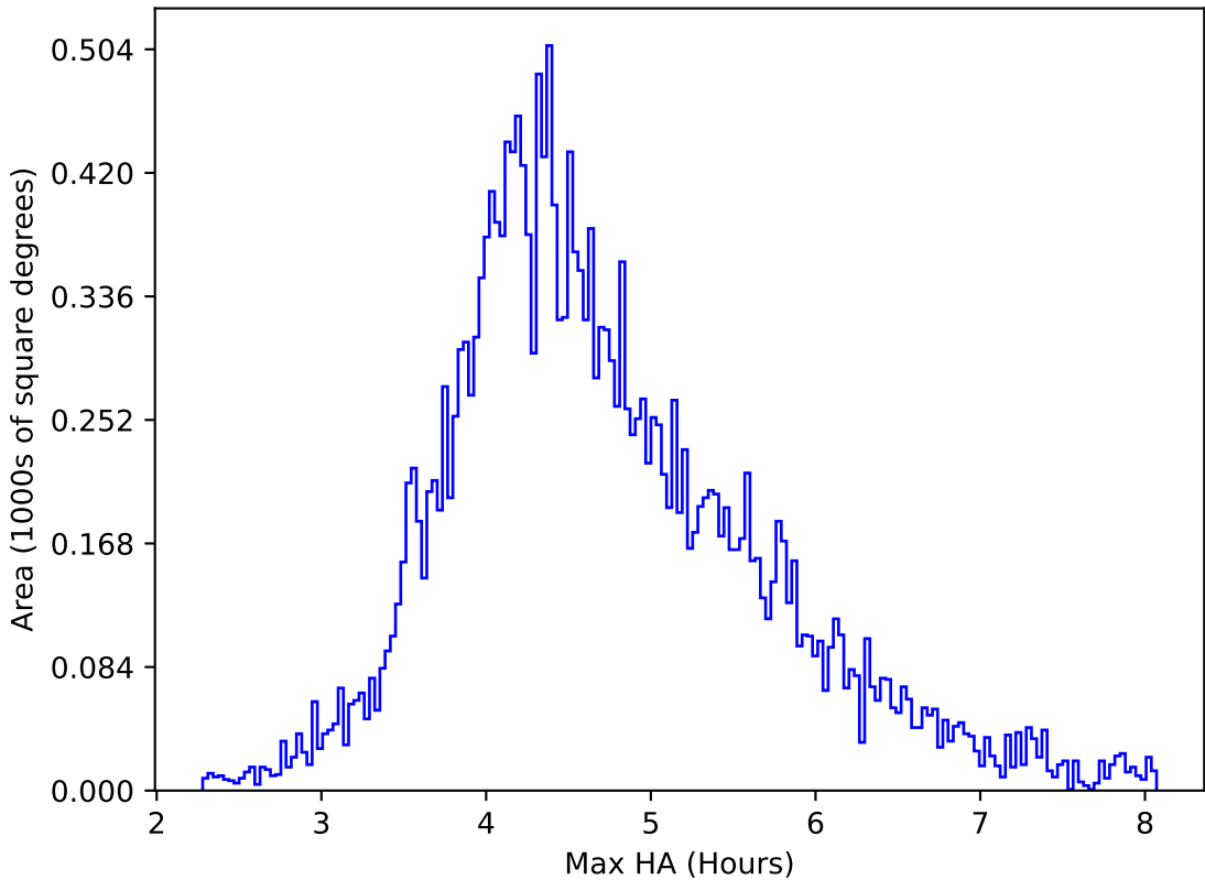
too_elab_heavy_r64_d2_gz_v3.4_10yrs All sky y band: Max HA
