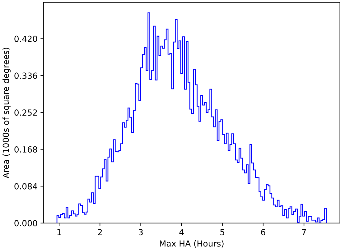
too_elab_heavy_r64_d2_gz_v3.4_10yrs All sky u band: Max HA
