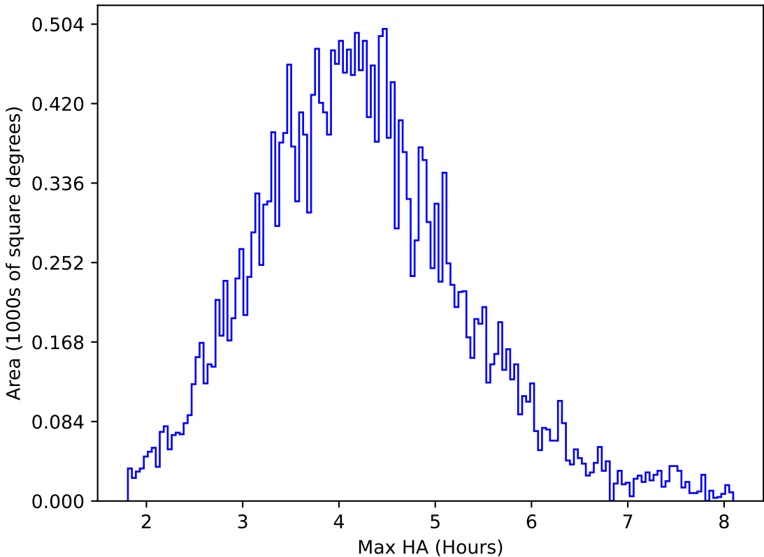
too_elab_heavy_r64_d2_gz_v3.4_10yrs All sky r band: Max HA
