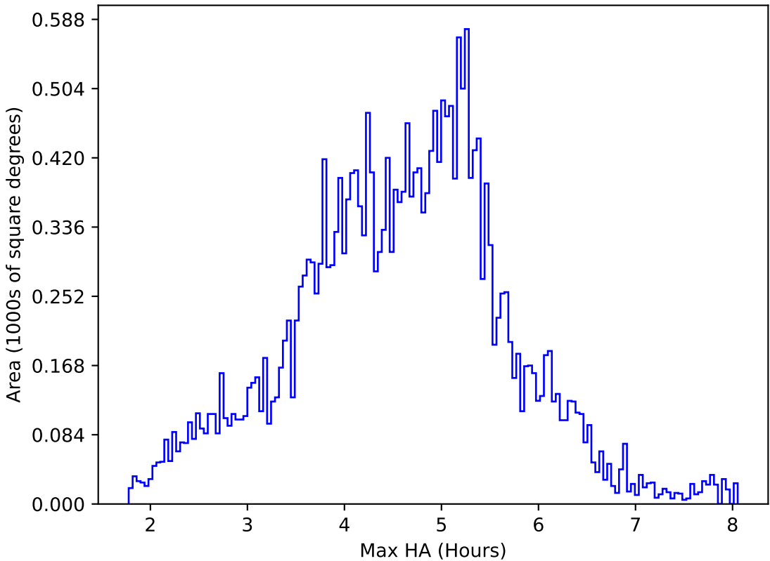
too_elab_heavy_r64_d2_gz_v3.4_10yrs All sky i band: Max HA
