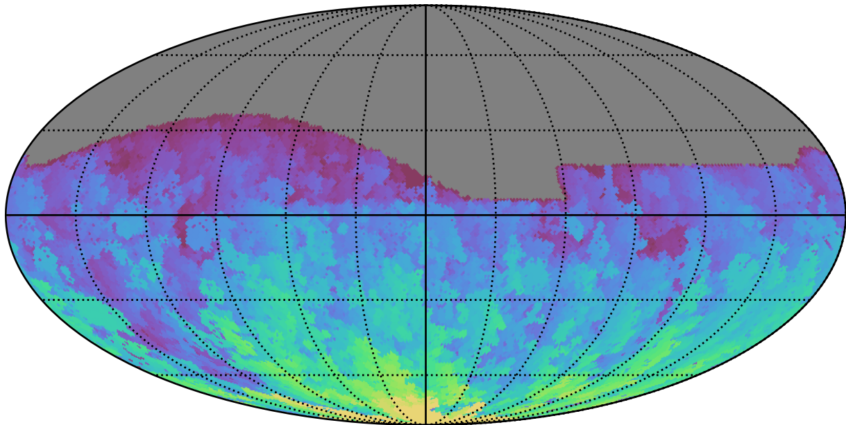
too_elab_heavy_r64_d2_gz_v3.4_10yrs All sky g band: Max HA
