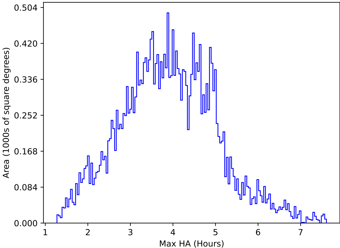
too_elab_heavy_r64_d2_gz_v3.4_10yrs All sky g band: Max HA
