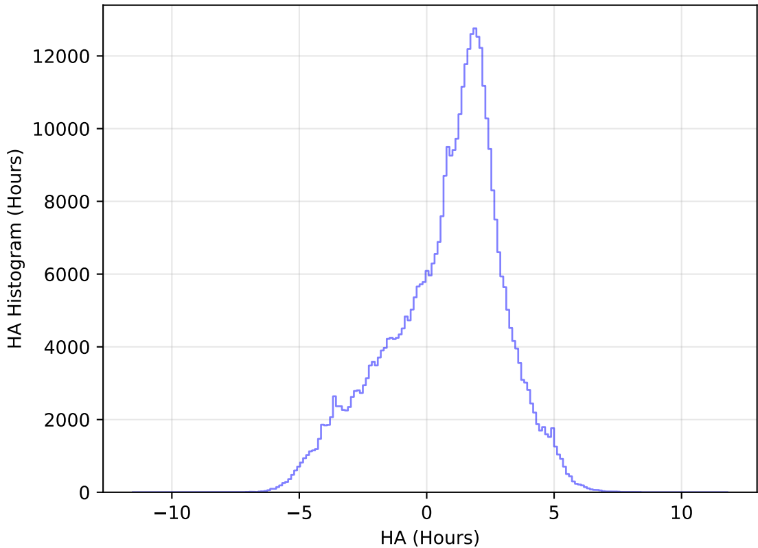
too_elab_heavy_r64_d2_gz_v3.4_10yrs WFD z band: HA Histogram
