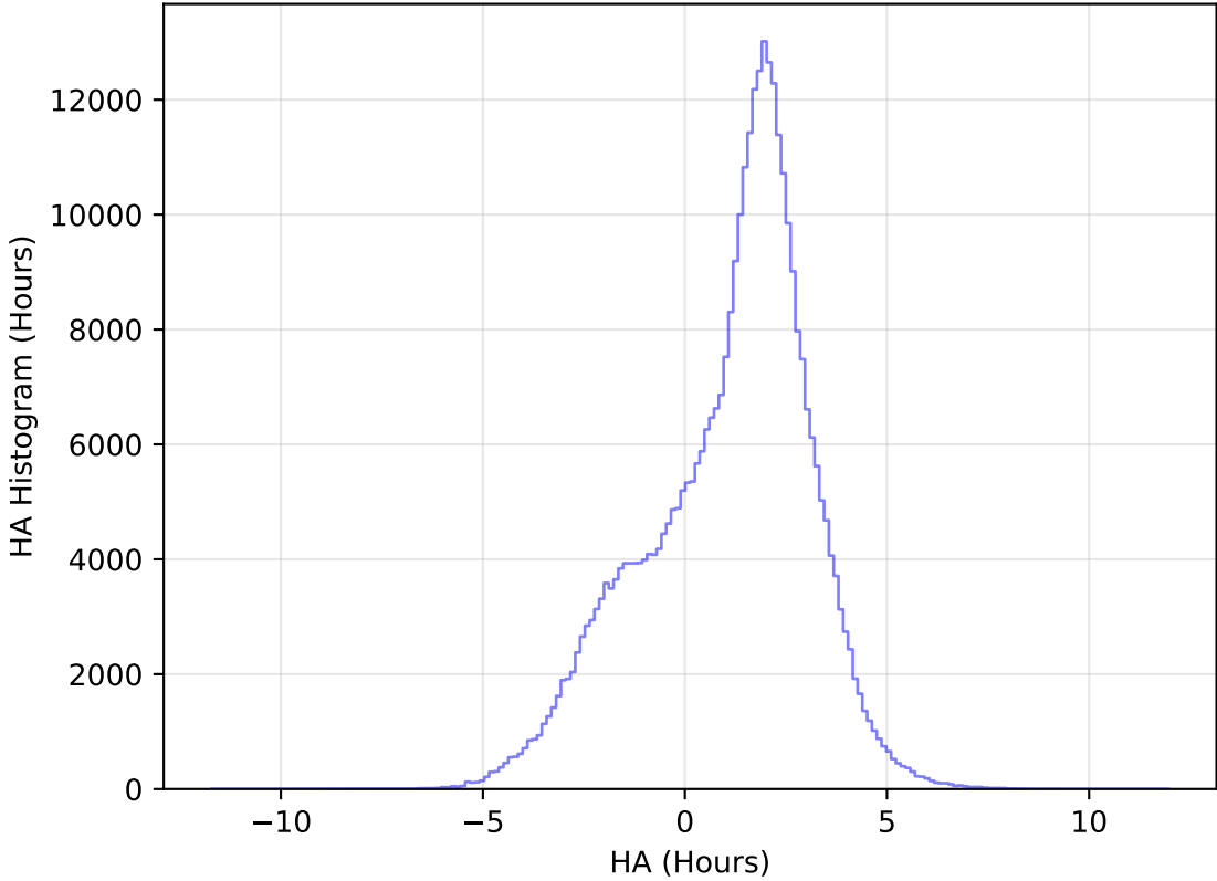
too_elab_heavy_r64_d2_gz_v3.4_10yrs WFD y band: HA Histogram
