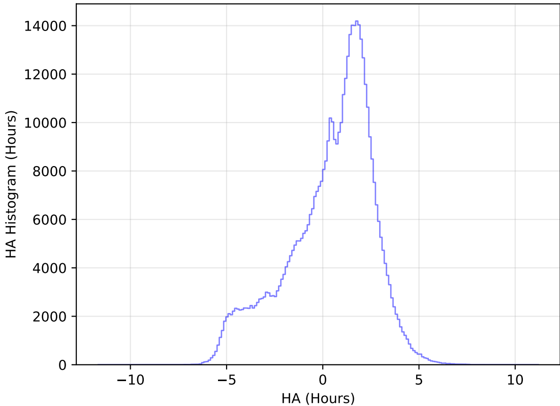
too_elab_heavy_r64_d2_gz_v3.4_10yrs WFD r band: HA Histogram
