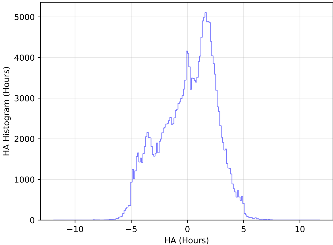
too_elab_heavy_r64_d2_gz_v3.4_10yrs WFD g band: HA Histogram
