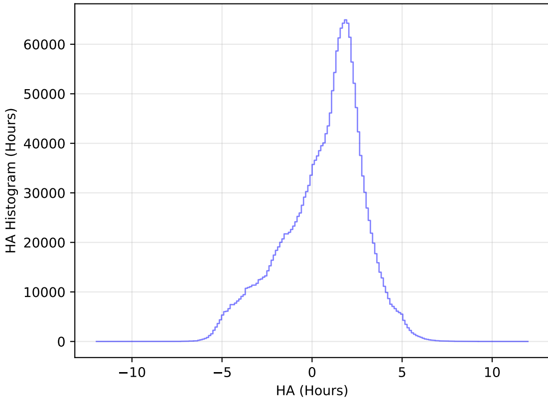
too_elab_heavy_r64_d2_gz_v3.4_10yrs WFD all bands: HA Histogram
