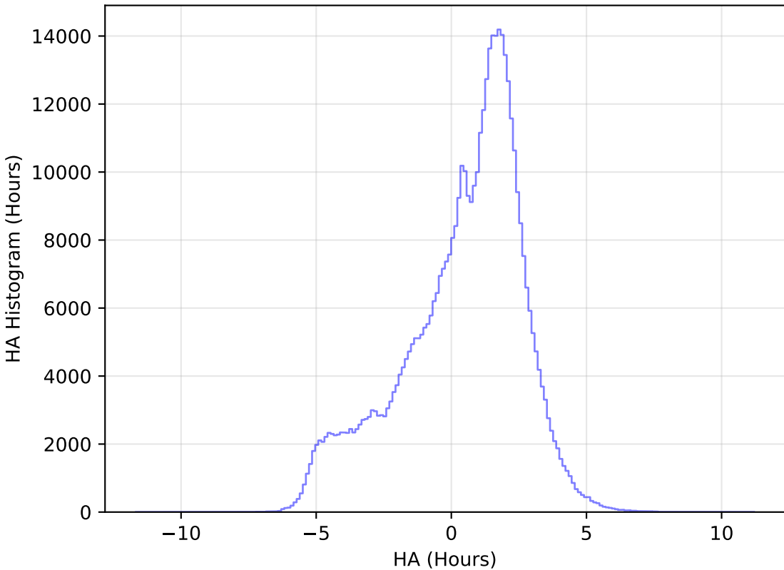
too_elab_heavy_r64_d2_gz_v3.4_10yrs All sky r band: HA Histogram
