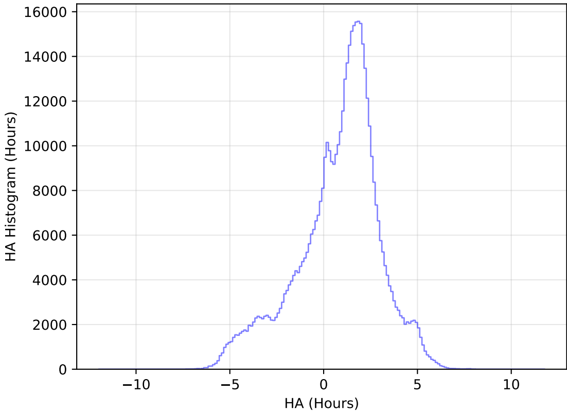
too_elab_heavy_r64_d2_gz_v3.4_10yrs All sky i band: HA Histogram
