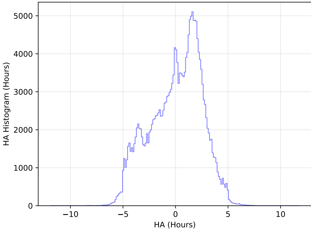
too_elab_heavy_r64_d2_gz_v3.4_10yrs All sky g band: HA Histogram
