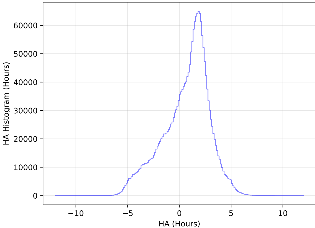
too_elab_heavy_r64_d2_gz_v3.4_10yrs All sky all bands: HA Histogram
