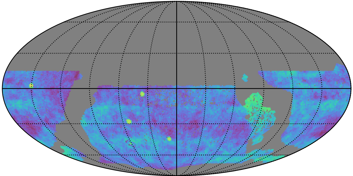
too_elab_heavy_r64_d2_gz_v3.4_10yrs gri WFD: Fraction of visits in pairs (20-90 min)
