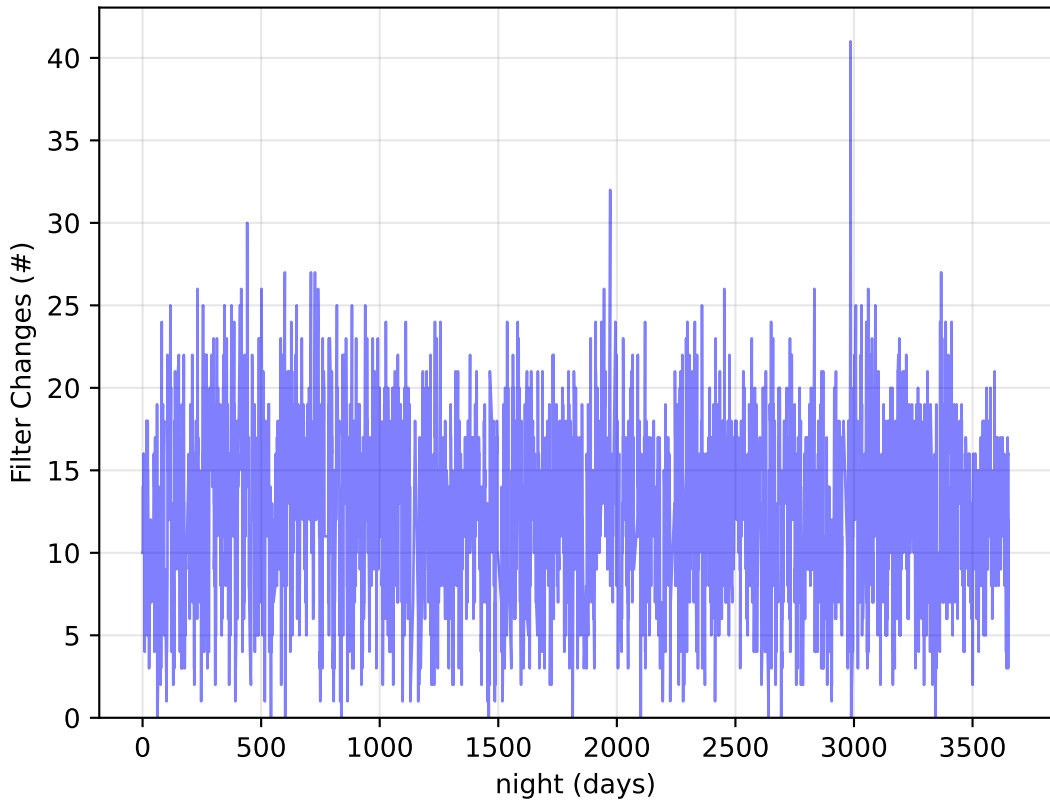
too_elab_heavy_r64_d2_gz_v3.4_10yrs Per Night: Filter Changes
