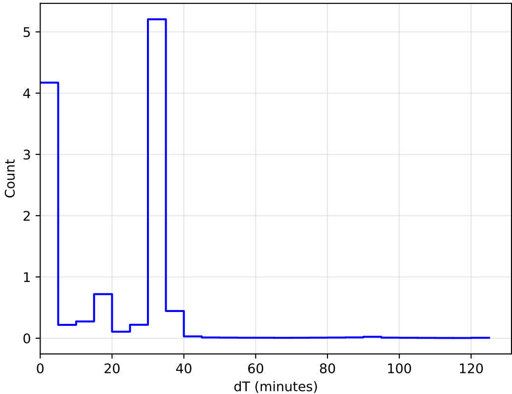
too_elab_heavy_r64_d2_gz_v3.4_10yrs WFD: DeltaT Histogram 1e6
