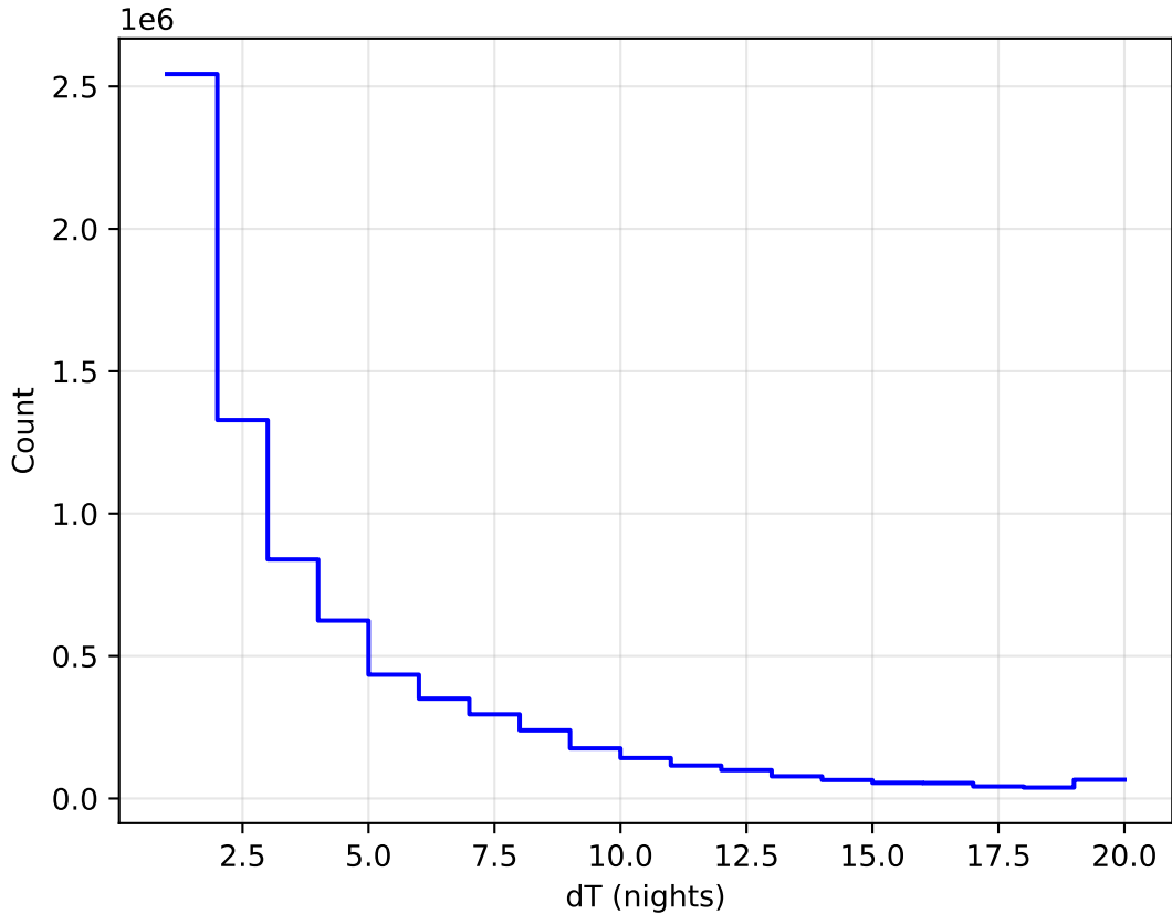
too_elab_heavy_r64_d2_gz_v3.4_10yrs WFD all bands: DeltaNight Histogram
