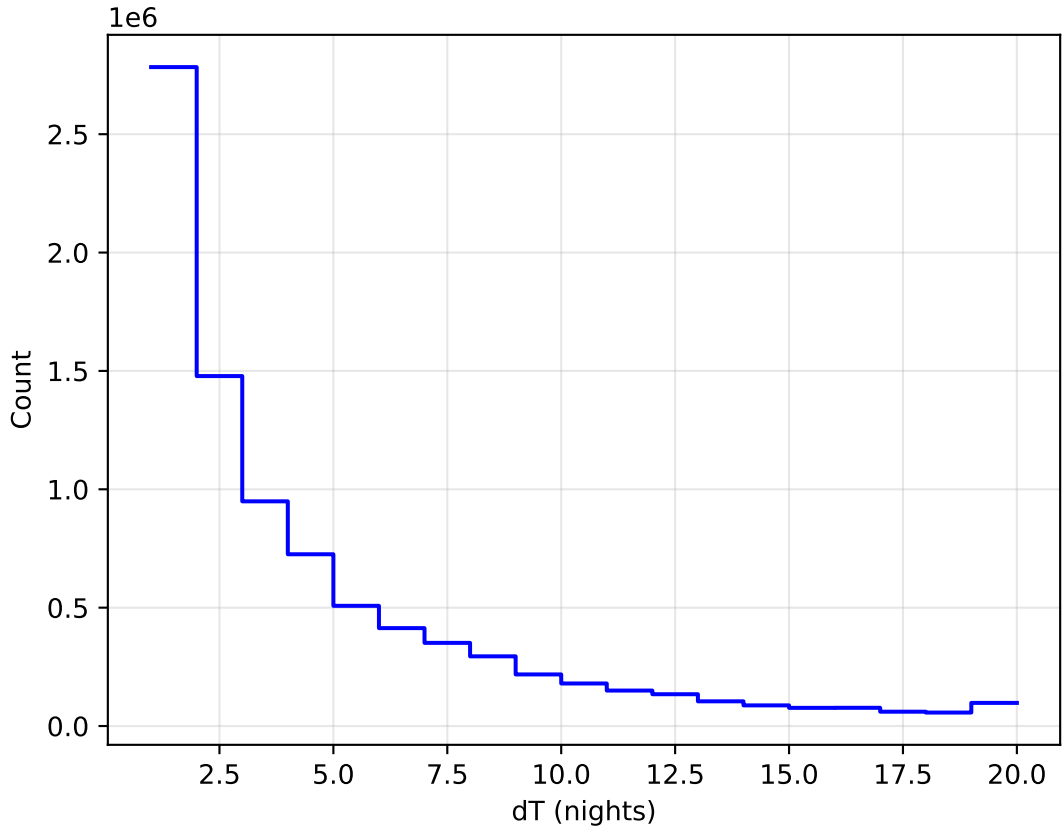
too_elab_heavy_r64_d2_gz_v3.4_10yrs All sky all bands: DeltaNight Histogram
