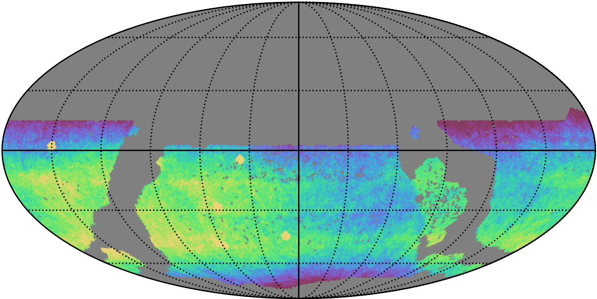
too_elab_heavy_r64_d2_gz_v3.4_10yrs WFD r band: CoaddM5
