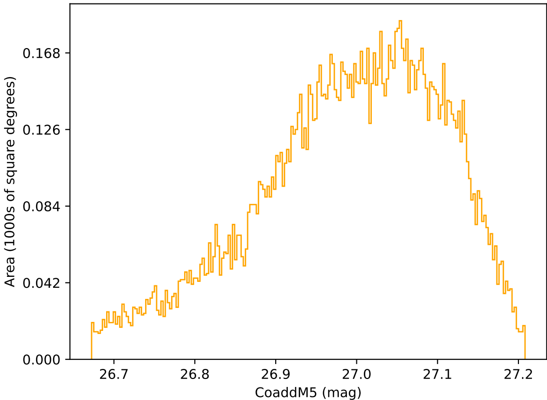
too_elab_heavy_r64_d2_gz_v3.4_10yrs WFD r band: CoaddM5
