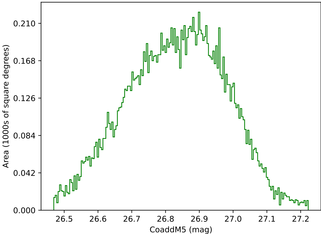
too_elab_heavy_r64_d2_gz_v3.4_10yrs WFD g band: CoaddM5
