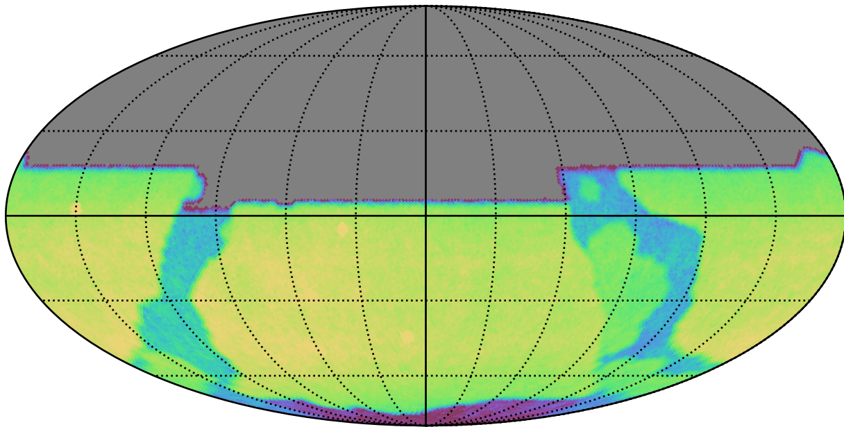
too_elab_heavy_r64_d2_gz_v3.4_10yrs All sky y band: CoaddM5
