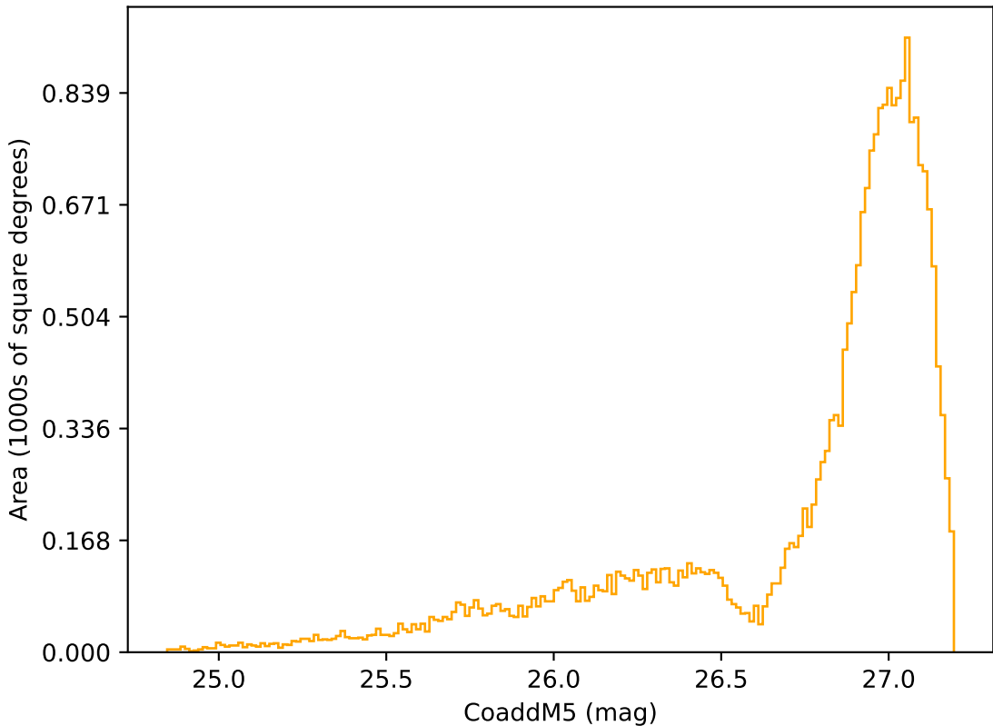
too_elab_heavy_r64_d2_gz_v3.4_10yrs All sky r band: CoaddM5
