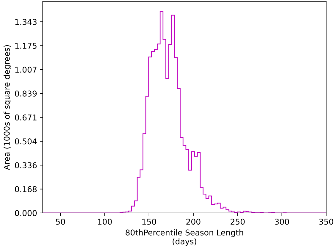
too_elab_heavy_r64_d2_gz_v3.4_10yrs WFD z band: 80thPercentile Season Length
