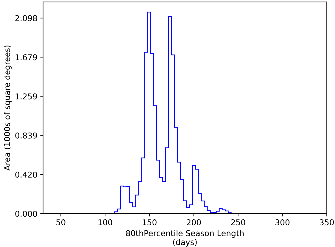
too_elab_heavy_r64_d2_gz_v3.4_10yrs WFD y band: 80thPercentile Season Length
