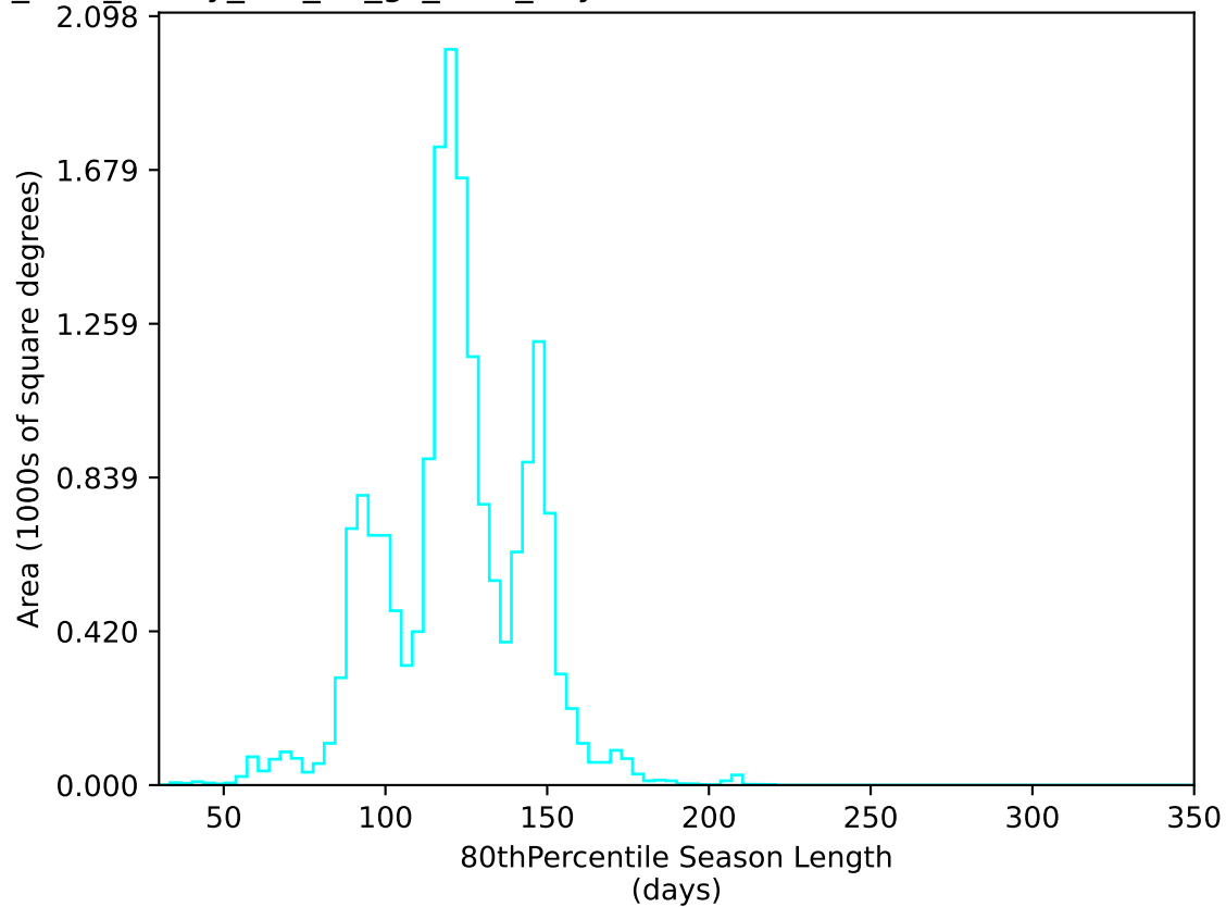
too_elab_heavy_r64_d2_gz_v3.4_10yrs WFD u band: 80thPercentile Season Length
