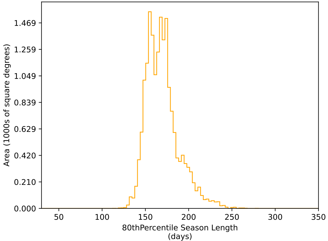
too_elab_heavy_r64_d2_gz_v3.4_10yrs WFD r band: 80thPercentile Season Length
