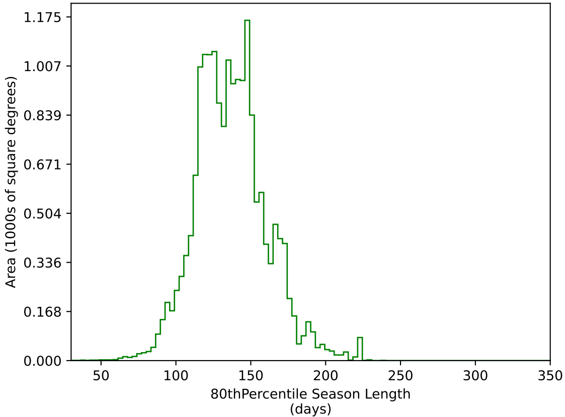
too_elab_heavy_r64_d2_gz_v3.4_10yrs WFD g band: 80thPercentile Season Length
