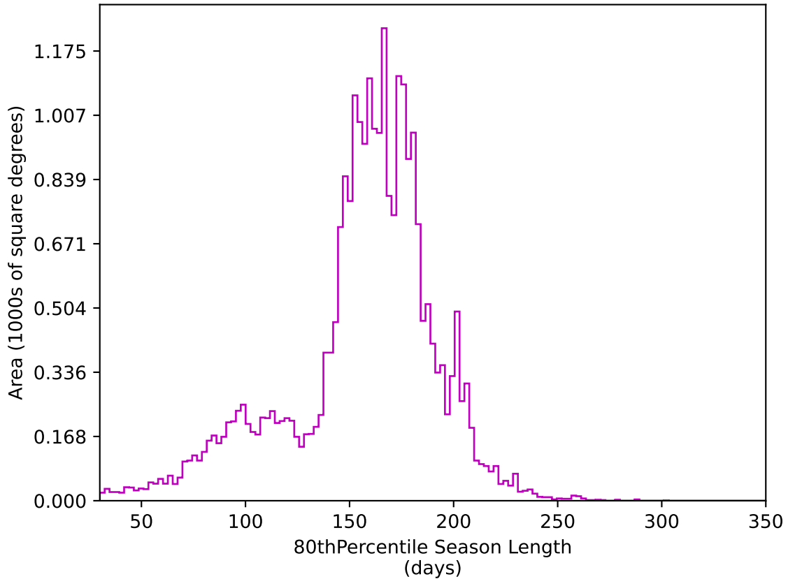
too_elab_heavy_r64_d2_gz_v3.4_10yrs All sky z band: 80thPercentile Season Length
