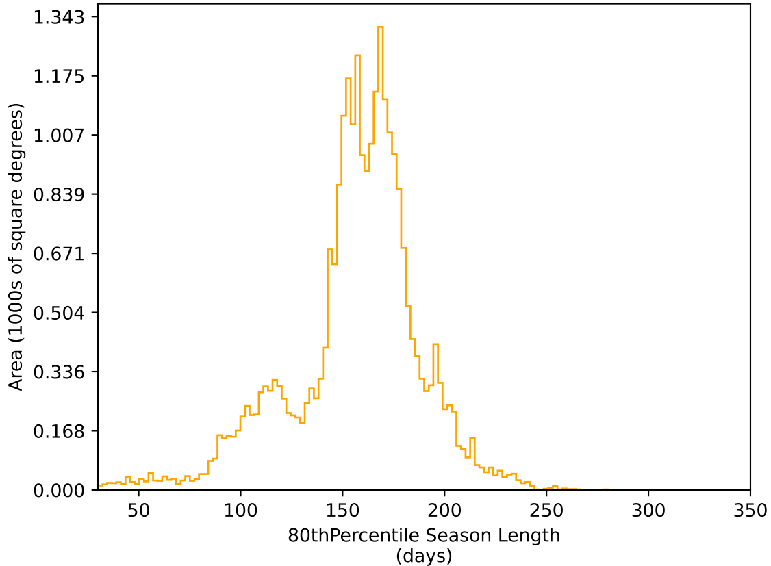
too_elab_heavy_r64_d2_gz_v3.4_10yrs All sky r band: 80thPercentile Season Length
