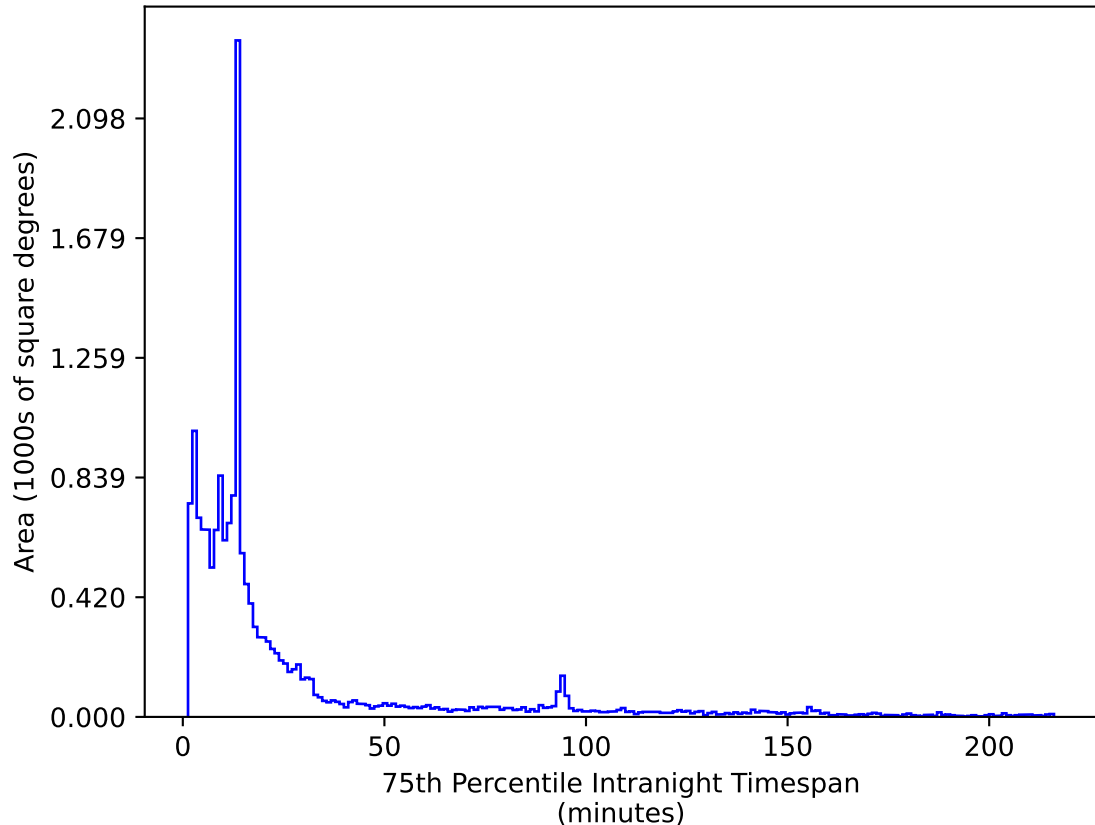
too_elab_heavy_r64_d2_gz_v3.4_10yrs WFD z band: 75th Percentile Intranight Timespan
