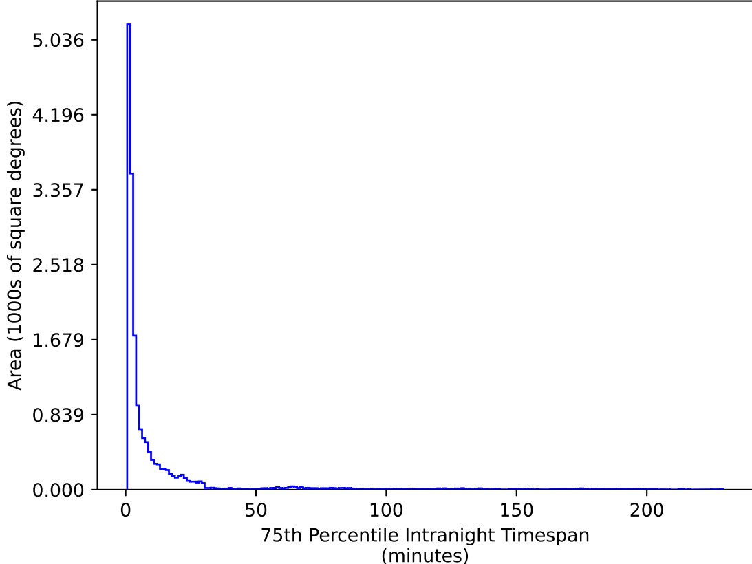
too_elab_heavy_r64_d2_gz_v3.4_10yrs WFD u band: 75th Percentile Intranight Timespan
