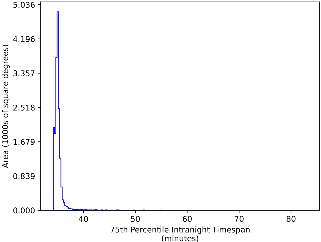
too_elab_heavy_r64_d2_gz_v3.4_10yrs WFD ri bands: 75th Percentile Intranight Timespan
