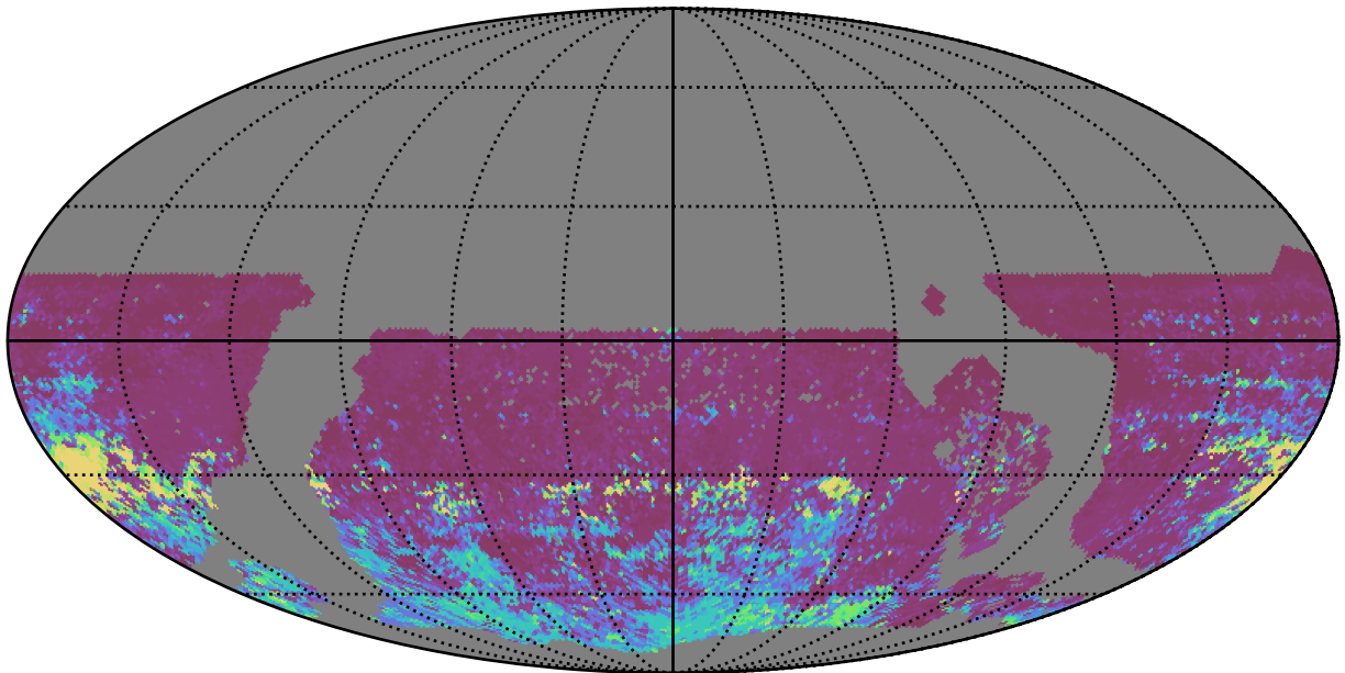
too_elab_heavy_r64_d2_gz_v3.4_10yrs WFD r band: 75th Percentile Intranight Timespan
