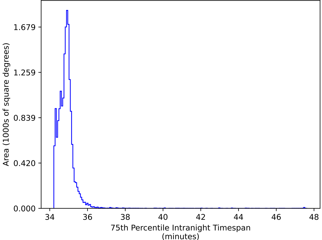
too_elab_heavy_r64_d2_gz_v3.4_10yrs WFD iz bands: 75th Percentile Intranight Timespan
